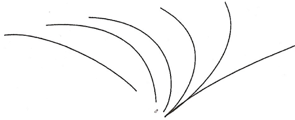
Figure 2-22a. Frame-by-frame sequence of a forward cast made by the author showing the broad Casting Arc needed to compensate for the deep rod load, or the deep rod load needed to compensate for the broad Casting Arc. Note the beginning and ending inclinations of the rod. (Author's data).
