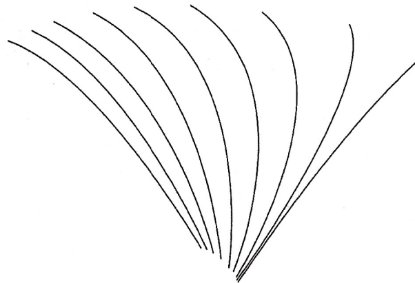
Figure 2-22b. Frame-by-frame sequence of a forward cast made by the author showing the narrow Casting Arc needed to complement shallow rod load, or the shallow rod load needed to complement the narrow Casting Arc. Note the beginning and ending inclinations of the rod. (Author's data).
