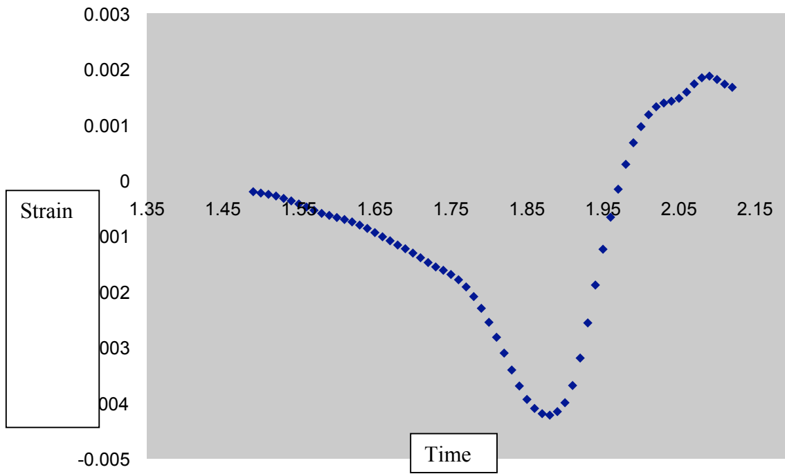
Fig.6 --Detailed strain vs time with good preload
